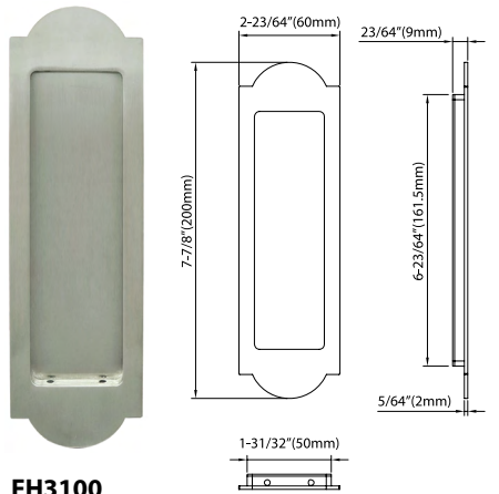
FH3100 Flush Pull Only
